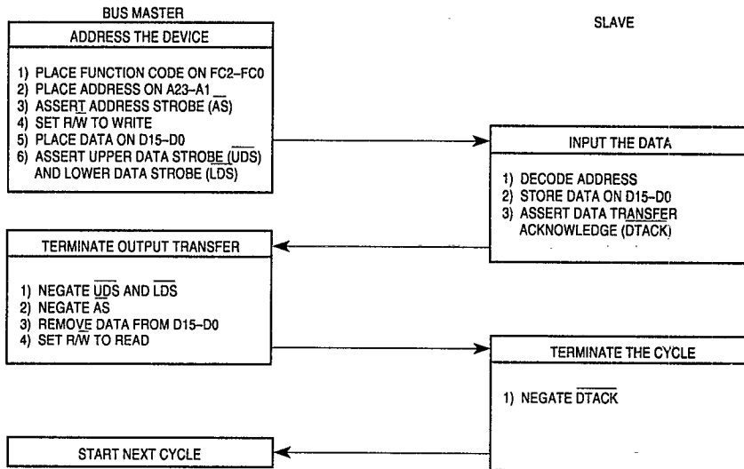
Figure 5-5. Word Write-Cycle Flowchart
