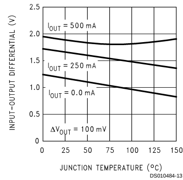
Dropout Voltage
