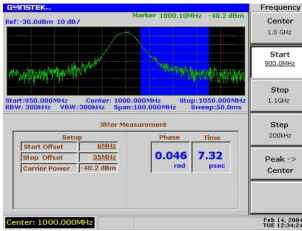
Jitter Measurement
