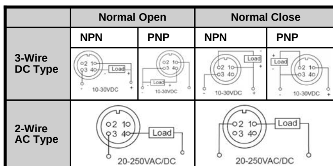
Quick Connector Type Wiring Diagram
