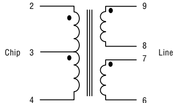
Schematic 3
