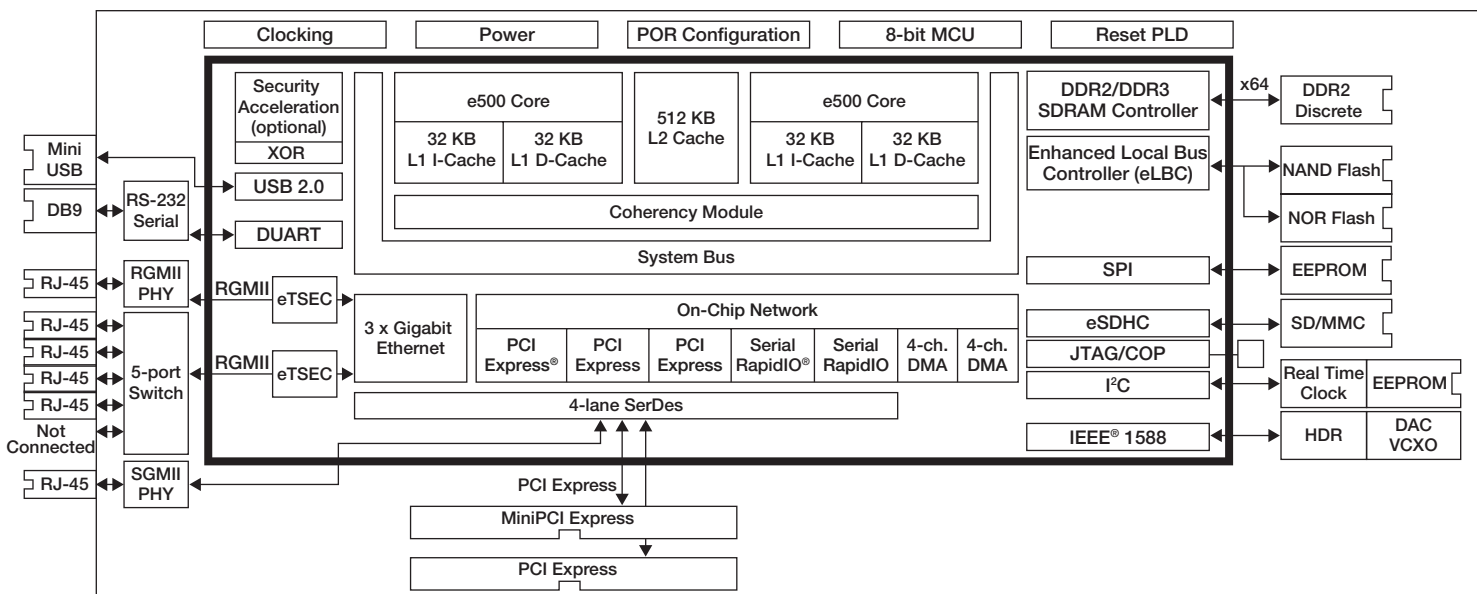
P2020RDB Block Diagram
