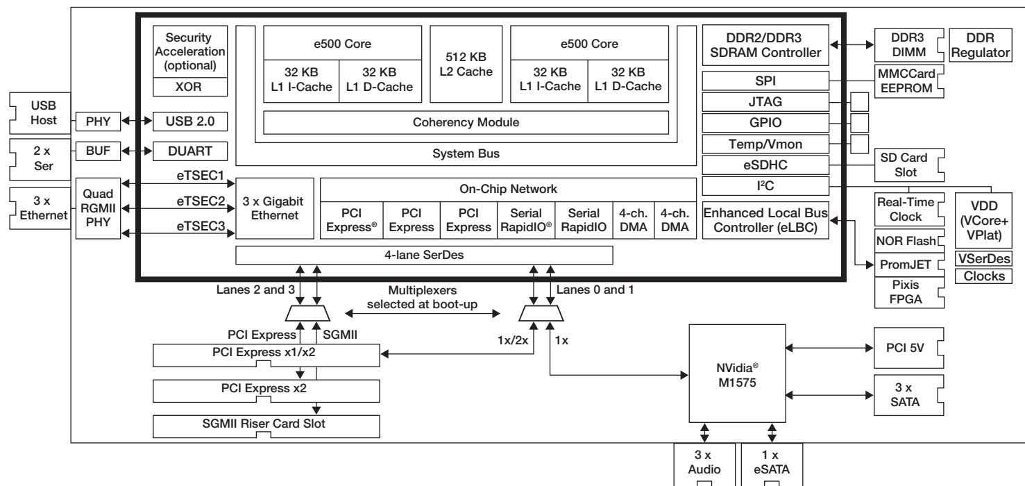
P2020DS Block Diagram
