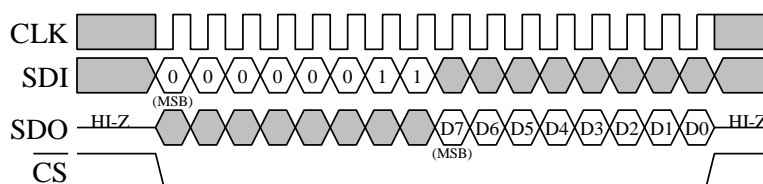
Figure 3 Timing Diagram for 8-Bit Control Register Read Operation
