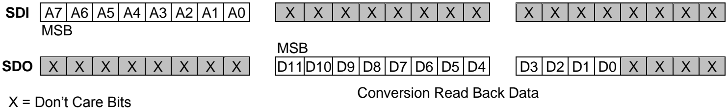
Figure 5 Register Diagram for 12-Bit ADC Read Operation
