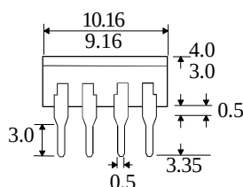
PS2505-4X PS2505-4
