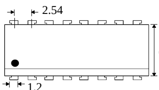
PS2505-4X PS2505-4
