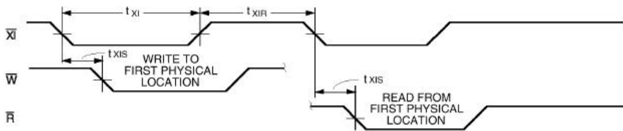
FIGURE 10. EXPANSION IN
