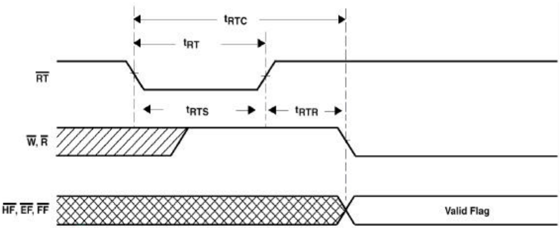
FIGURE 5. RETRANSMIT
