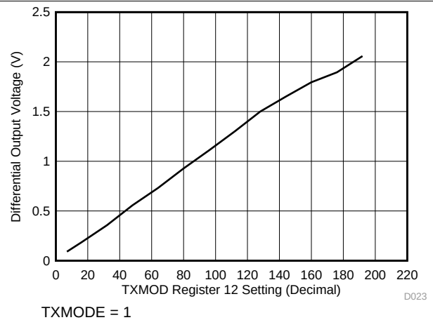
Figure 16. Output Voltage vs Modulation Current
