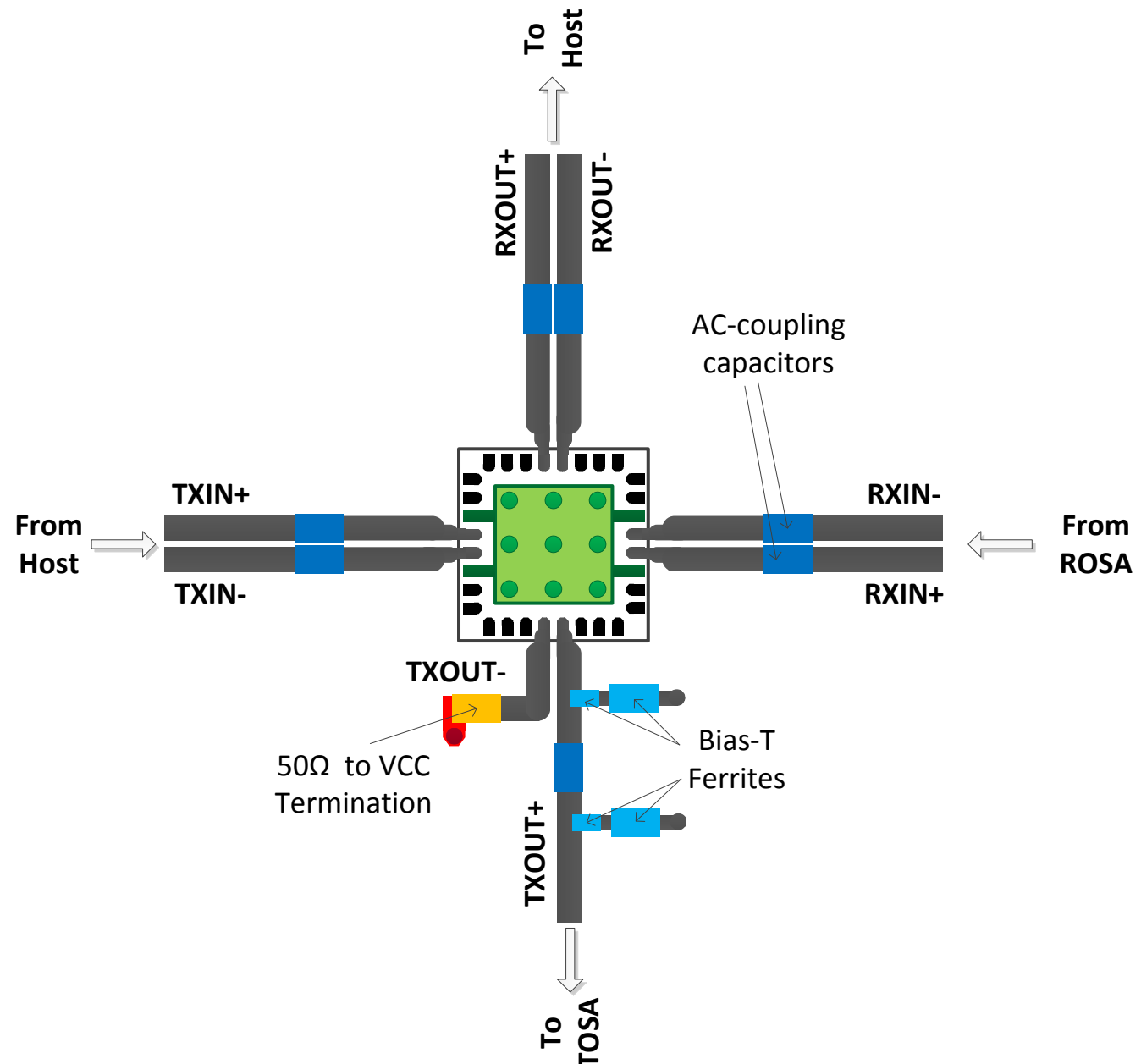
Figure 73. Board Layout
