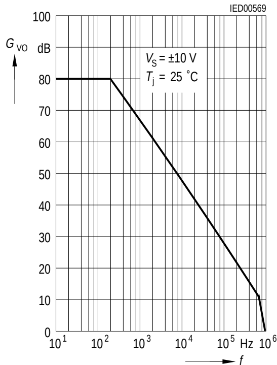
TCA 2465, G Open-Loop Voltage Gain versus Frequency V_S = \pm 10 \text{ V}, T_j = 25 \text{ }^\circ\text{C}
