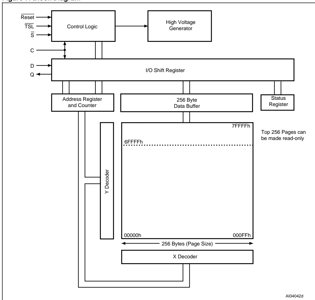
Figure 7. Block Diagram
