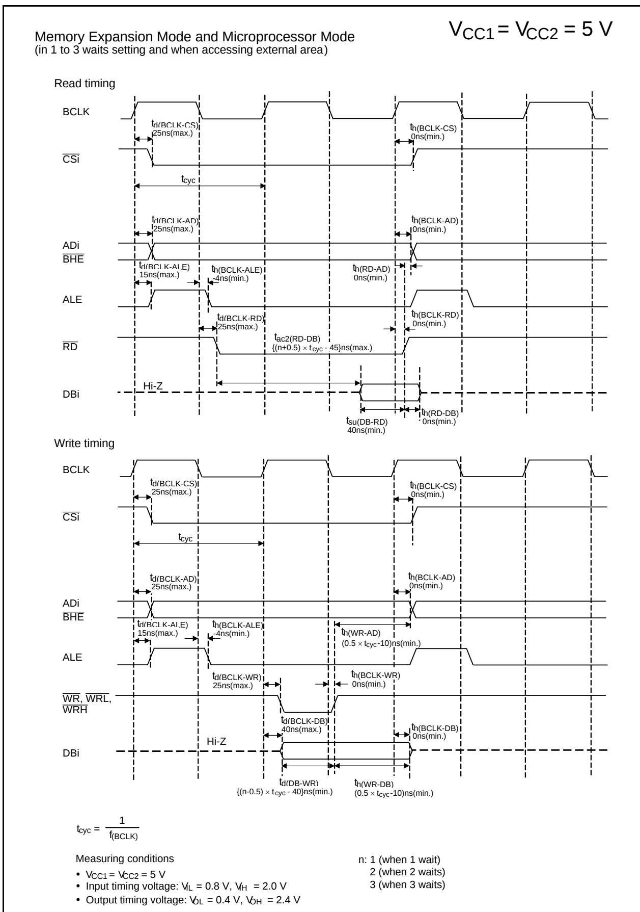
Figure 5.15 Timing Diagram
