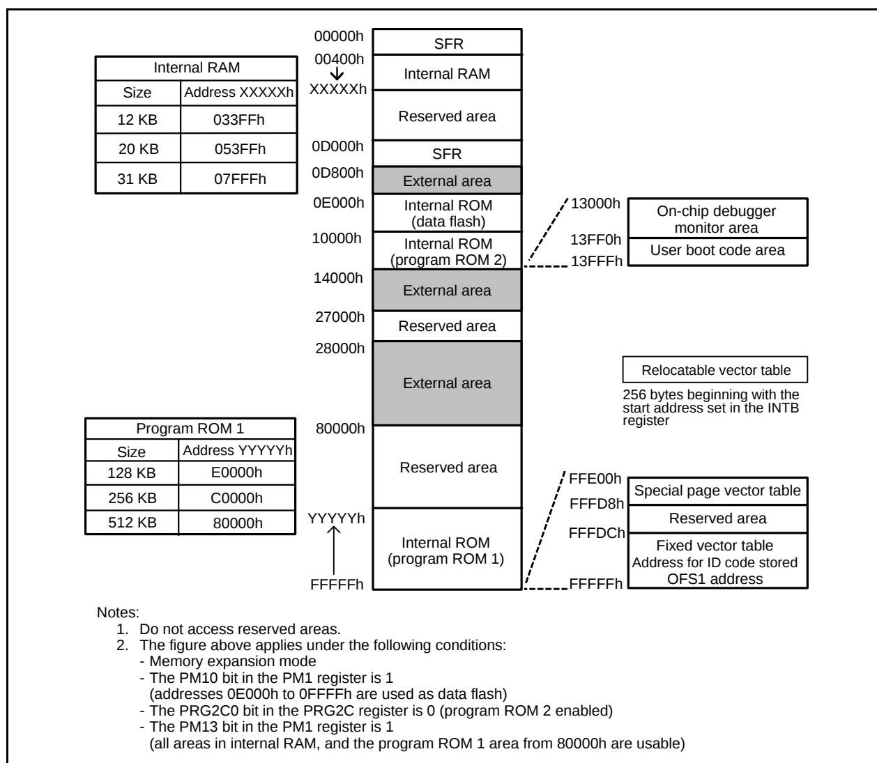
Figure 3.2 Memory Map
