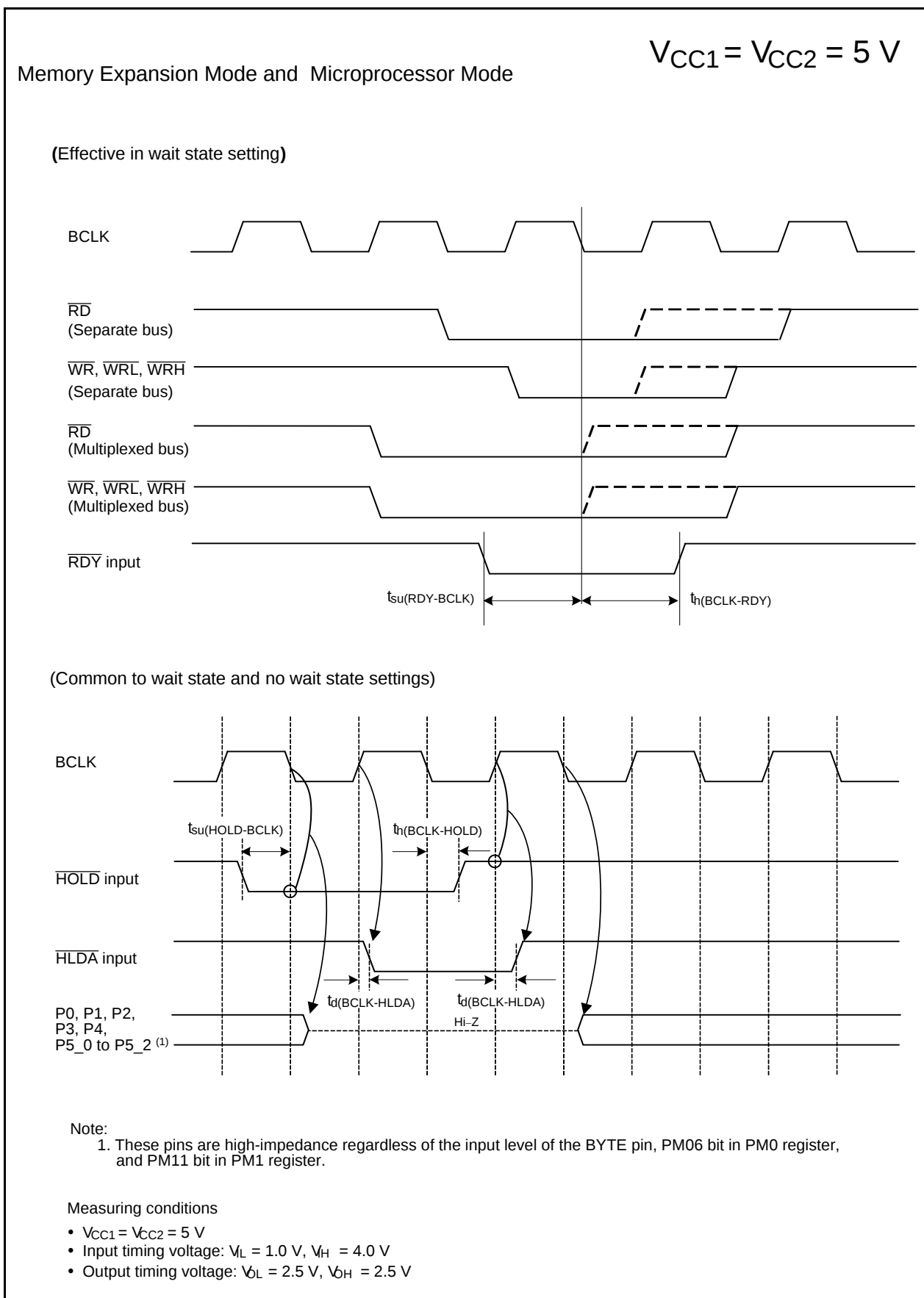
Figure 5.12 Timing Diagram
