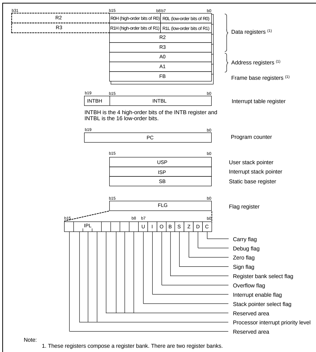
Figure 2.1 CPU Register
