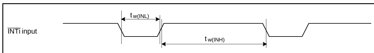
Figure 5.23 External Interrupt \overline{\text{INTi}} Input
