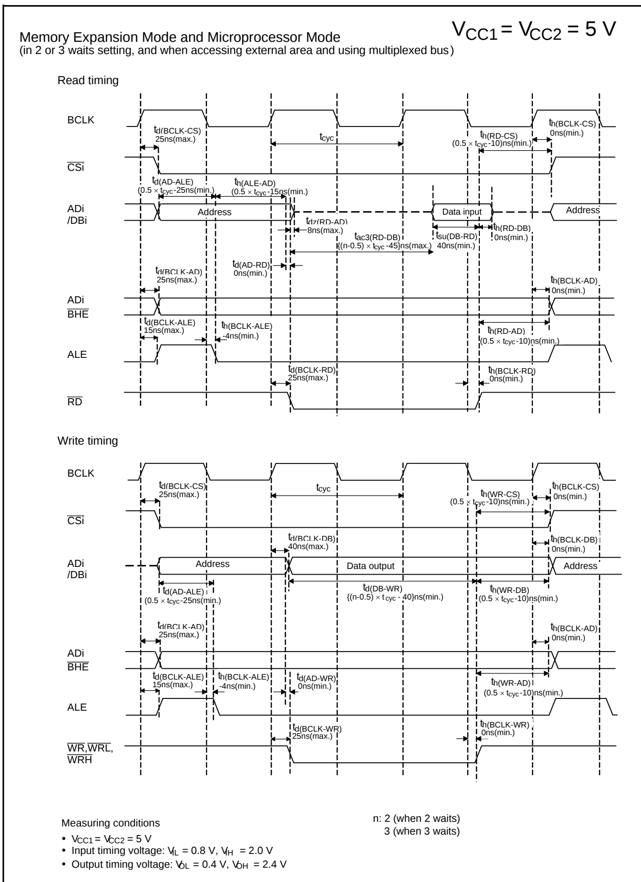
Figure 5.16 Timing Diagram
