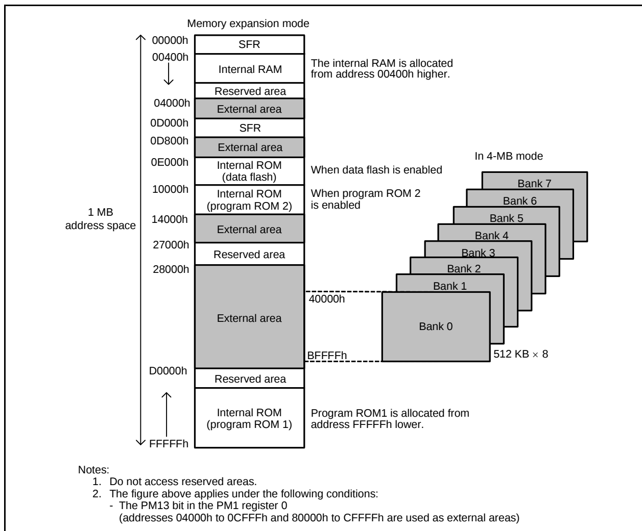
Figure 3.1 Address Space
