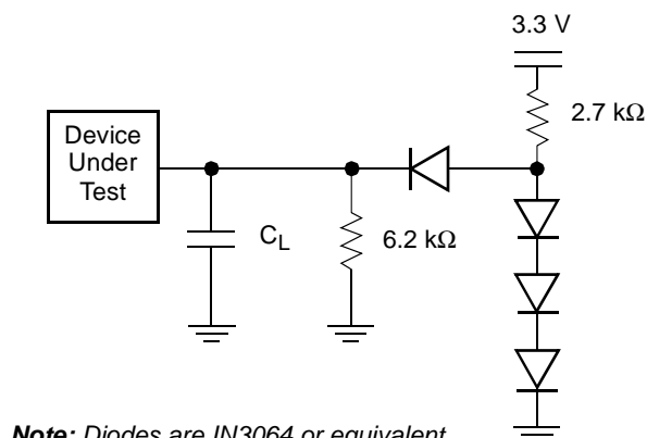
Figure 12. Test Setup
