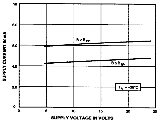
SUPPLY CURRENT
