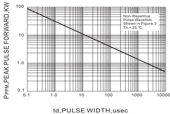
Fig. 1 PEAK PULSE POWER RATING VERSUS PULSE TIME CURVE
