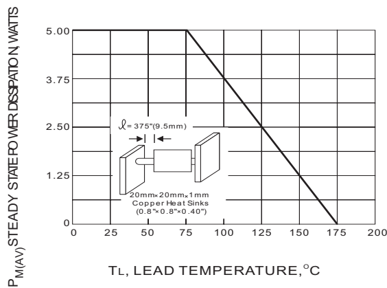
Fig. 5 STEADY STATE POWER DERATING
