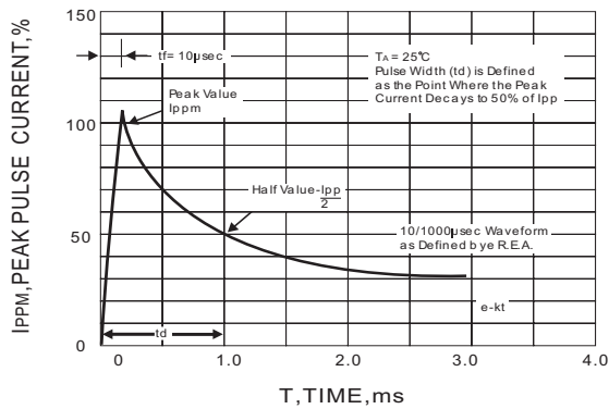
Fig. 3 PULSE WAVEFORM
