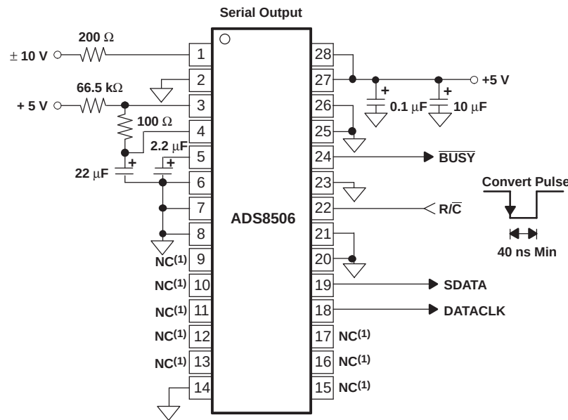
Figure 32. Basic \pm 10\text{-V} Operation With Serial Output
