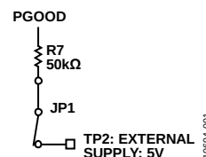
Figure 2 PGOOD Signal
