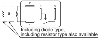
Schematic (Bottom view) 1 Form A
