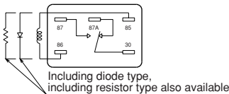
1 Form C
