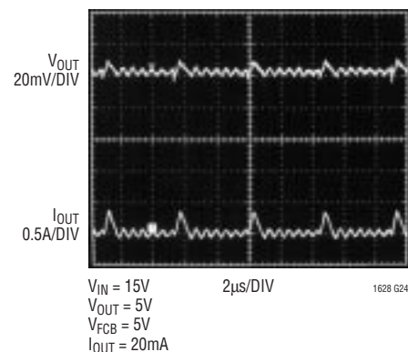
Constant Frequency (Burst Inhibit) Operation (Figure 13)
