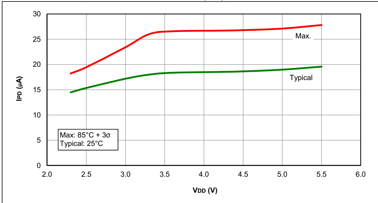
FIGURE 30-36: I_{PD} , FIXED VOLTAGE REFERENCE (FVR), PIC16F1508/9 ONLY
