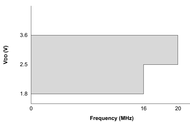
FIGURE 29-2: VOLTAGE FREQUENCY GRAPH, -40^{\circ}\text{C} \leq T_A \leq +125^{\circ}\text{C} , PIC16LF1508/9 ONLY
