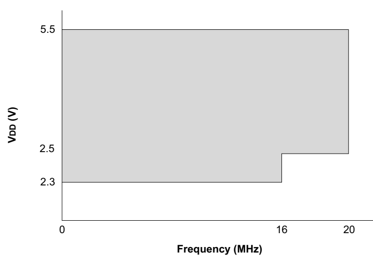
FIGURE 29-1: VOLTAGE FREQUENCY GRAPH, -40^{\circ}\text{C} \leq T_A \leq +125^{\circ}\text{C} , PIC16F1508/9 ONLY
