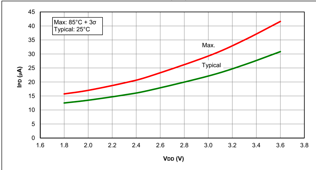
FIGURE 30-35: I_{PD} , FIXED VOLTAGE REFERENCE (FVR), PIC16LF1508/9 ONLY
