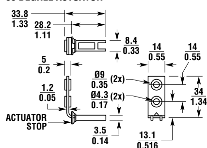
FLEX 1 AND FLEX 2 ACTUATORS
