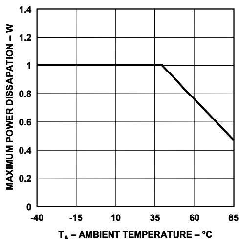
Figure 31. Power derating vs. temperature.
