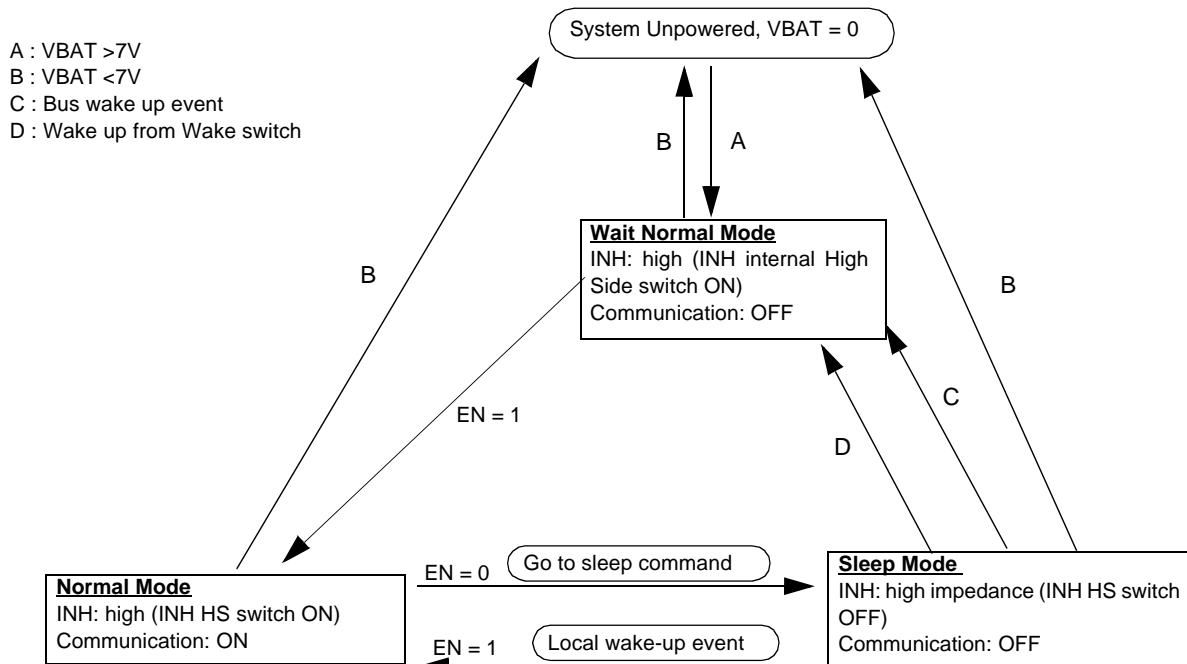
Figure 4. Device State Machine
