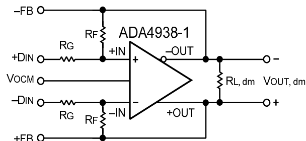
Figure 4. Circuit Definitions
