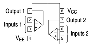
(Dual, Top View)
