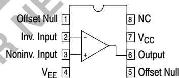
(Single, Top View)
