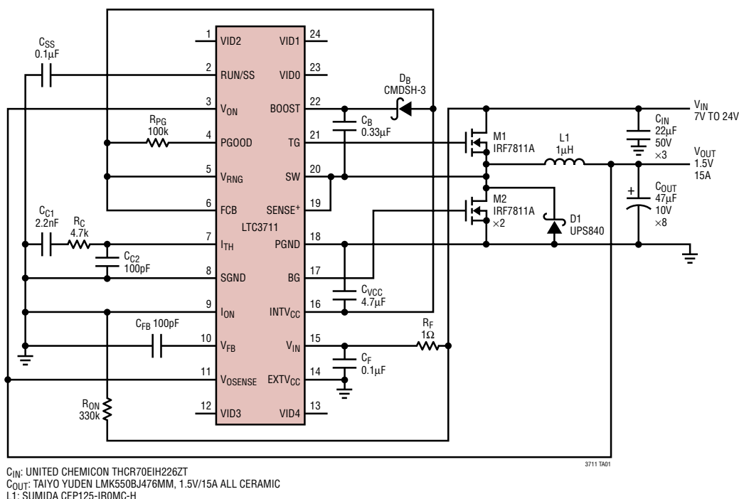
1.5V/15A All Ceramic C OUT
