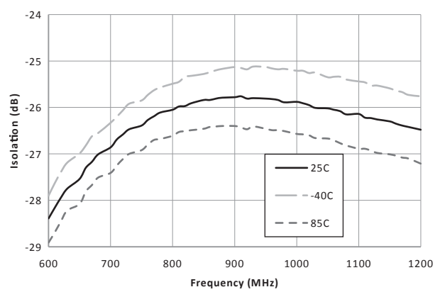
Figure 25. Isolation vs Frequency and Temperature
