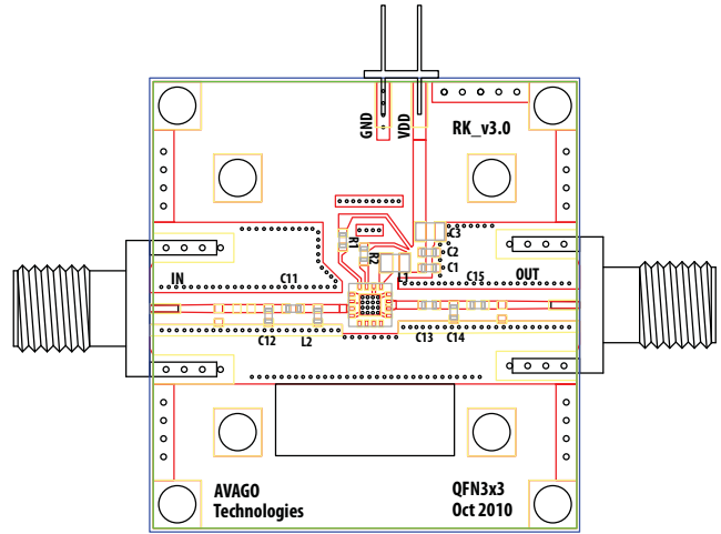
Figure 47. Demoboard
