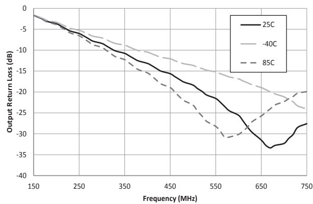
Figure 11. ORL vs Frequency and Temperature
