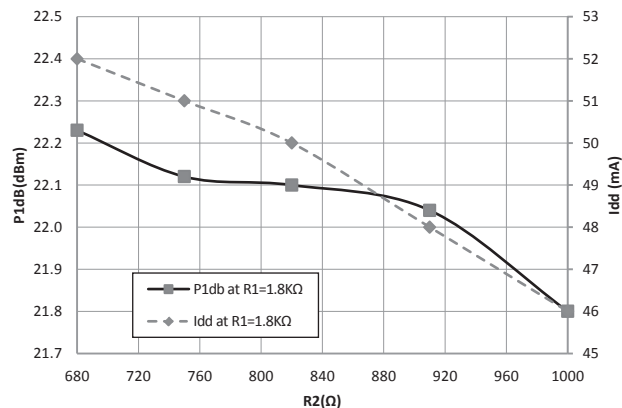
Figure 45. P1dB and Quiescent current with different R2 [1]
