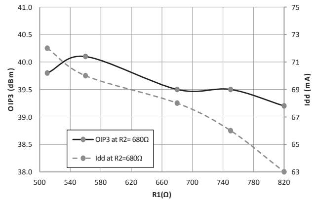
Figure 29. OIP3 and Quiescent current with different R1 [1]
