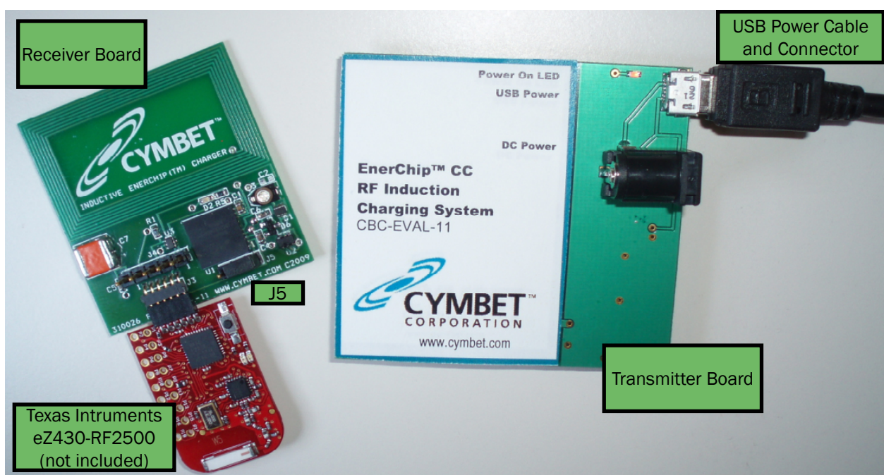
Figure 3: CBC-EVAL-11 Evaluation Kit.
