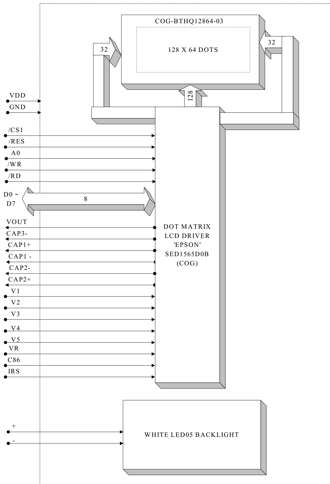
Figure 2: Block Diagram
