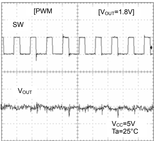
Figure 15. SW Waveform
