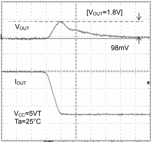
Figure 17. Transient Response ( I_o=600mA to 100mA , 10\mu s )
