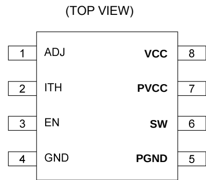
Figure 2. Pin Configuration
