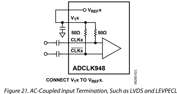
Figure 21. AC-Coupled Input Termination, Such as LVDS and LEVPECL
