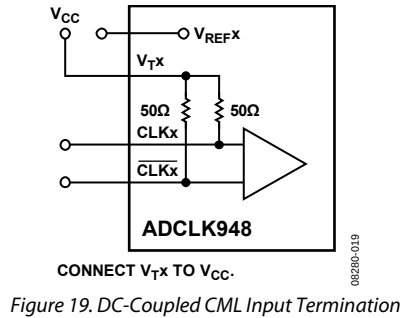
Figure 19. DC-Coupled CML Input Termination
