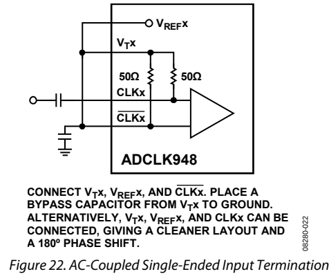
Figure 22. AC-Coupled Single-Ended Input Termination
