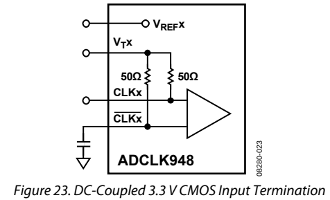
Figure 23. DC-Coupled 3.3 V CMOS Input Termination
