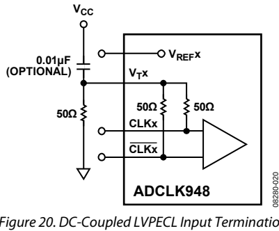
Figure 20. DC-Coupled LVPECL Input Termination
