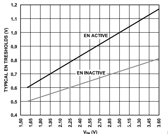
Figure 28. Typical EN Pin Thresholds vs. Input Voltage
