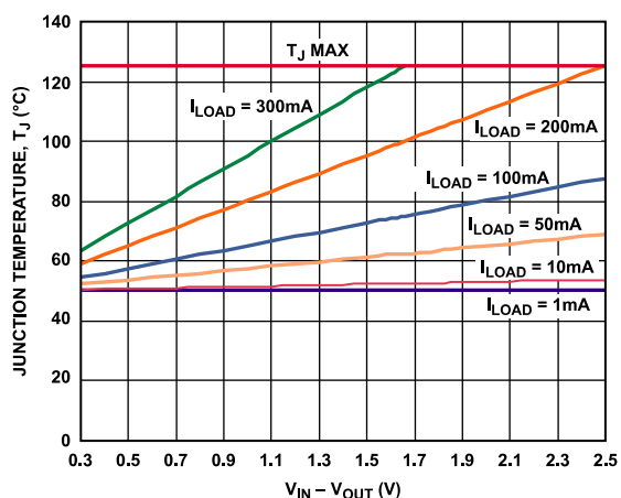
Figure 33. 500 mm² of PCB Copper, T_A = 50^\circ\text{C}
