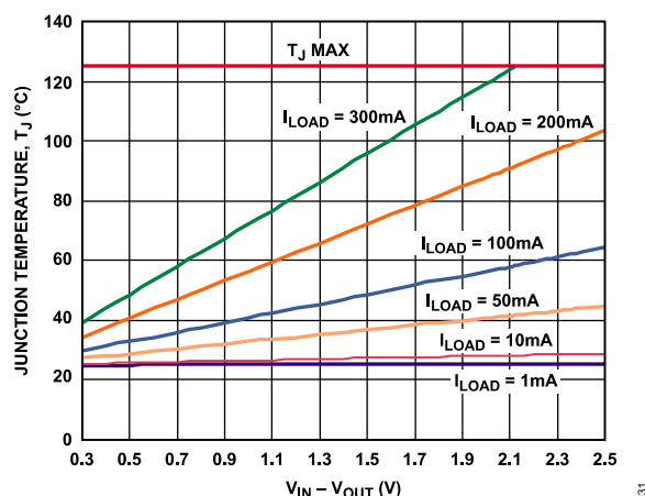
Figure 31. 100 mm 2 of PCB Copper, T_A = 25^\circ\text{C}
