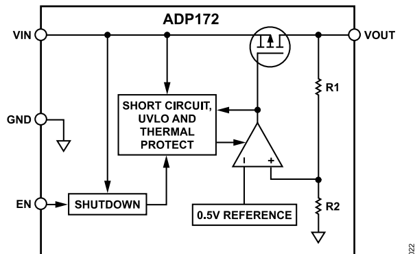
Figure 23. ADP172 Internal Block Diagram
