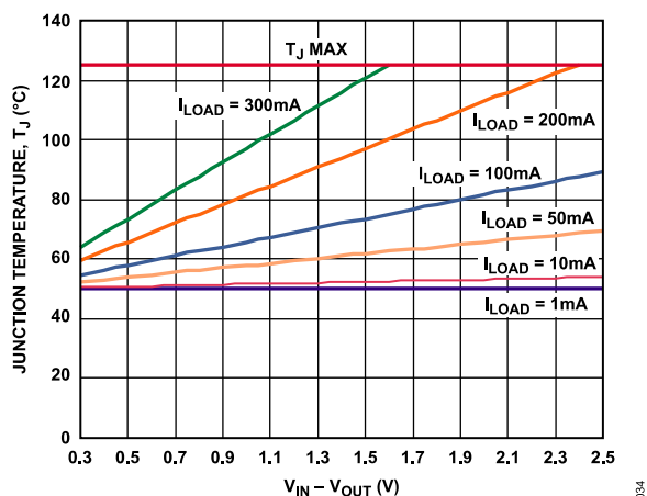
Figure 34. 100 mm² of PCB Copper, T_A = 50^\circ\text{C}
