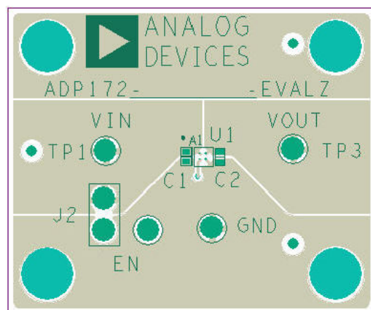
Figure 37. Example ADP172 PCB Layout
