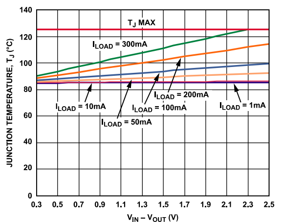
Figure 36. T_A = 85^\circ\text{C}
