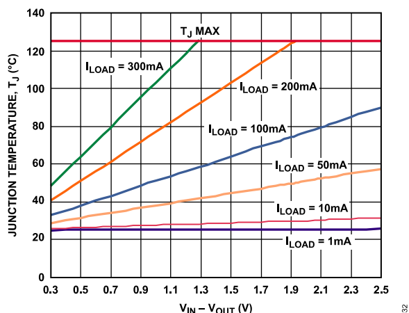
Figure 32. 0 mm² of PCB Copper, T_A = 25^\circ\text{C}
