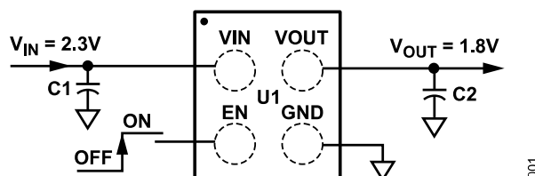
Figure 1. ADP172 with Fixed Output Voltage, 1.8 V
