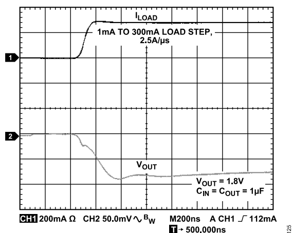
Figure 24. Output Transient Response, C_{OUT} = 1 \mu\text{F}
