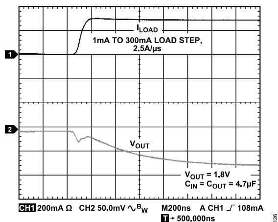
Figure 25. Output Transient Response, C_{OUT} = 4.7 \mu\text{F}
