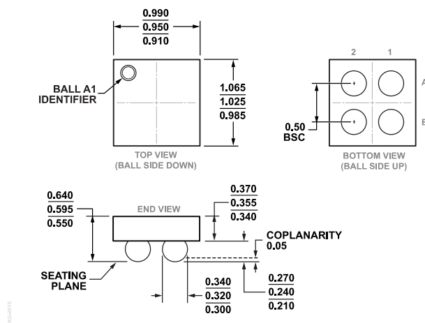
Figure 38. 4-Ball Wafer Level Chip Scale Package [WLCSP] (CB-4-4) Dimensions shown in millimeters
