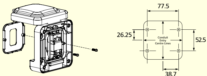
Fixing dimensions
