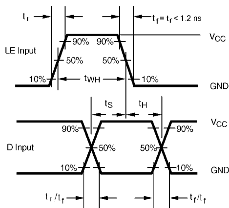
FIGURE 5. AC Waveforms
