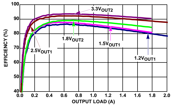
FIGURE 4. EFFICIENCY vs LOAD, 2.25MHz, 5VIN PWM
