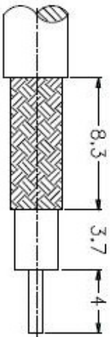
RECOMMENDED CABLE STRIPPING DIM'S
