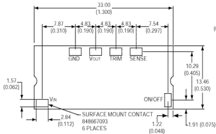
BOTTOM VIEW OF BOARD
