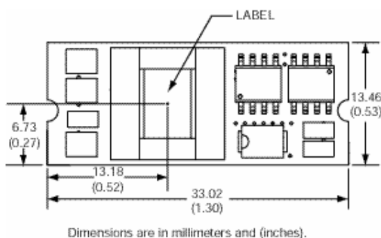
Figure 33. Pick and Place Location.
