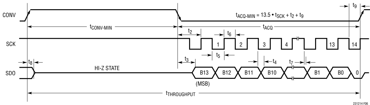
Figure 6. LTC2312-14 Serial Interface Timing Diagram (SCK High During t_{\text{CONV}} )
