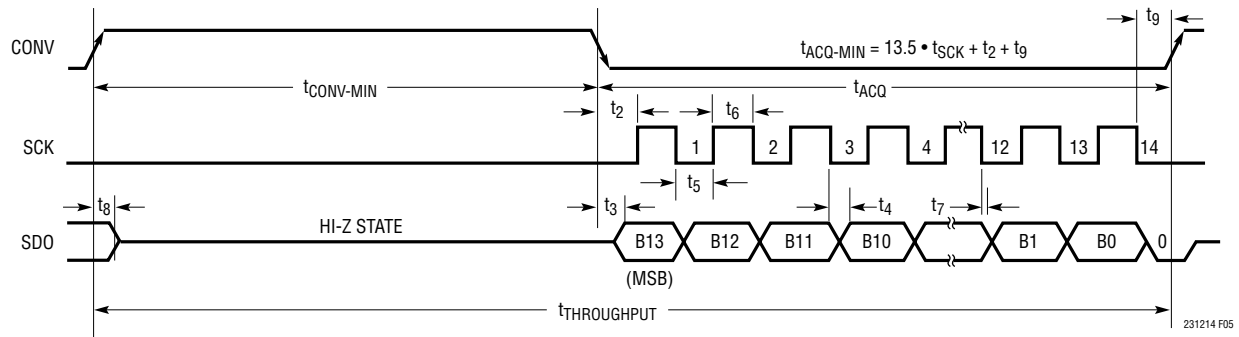
Figure 5. LTC2312-14 Serial Interface Timing Diagram (SCK Low During t_{\text{CONV}} )
