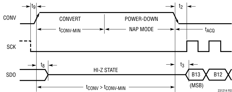
Figure 7. LTC2312-14 Nap Mode Power-Down Following Conversion for t_{\text{CONV}} > t_{\text{CONV-MIN}}
