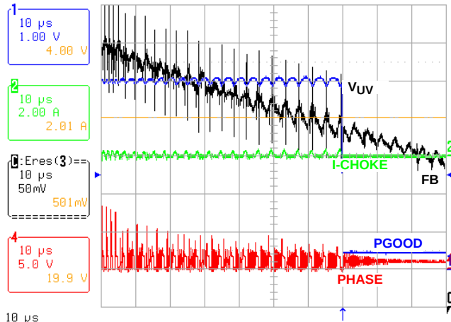
FIGURE 15. UNDERVOLTAGE PROTECTION: SHORT ACROSS HIGH-SIDE MOSFET GATE-SOURCE, 2A DC STATIC LOAD
