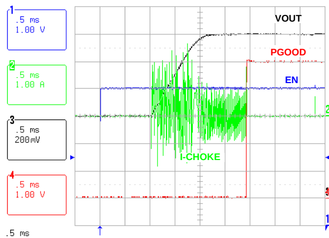
FIGURE 4. IN-RUSH CURRENT: NO LOAD, 50% VOUT-PREBIAS
