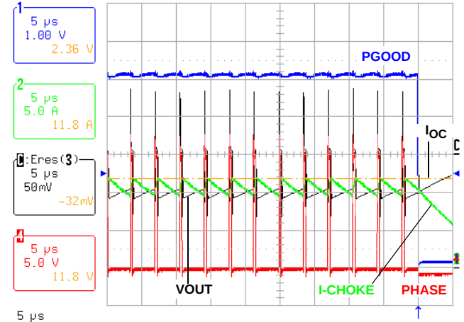
FIGURE 16. OVERCURRENT PROTECTION: 11.8A PEAK CHOKE CURRENT, 5.0mΩ r_{DS(ON)} , 2.1kΩ R_{SEN}
