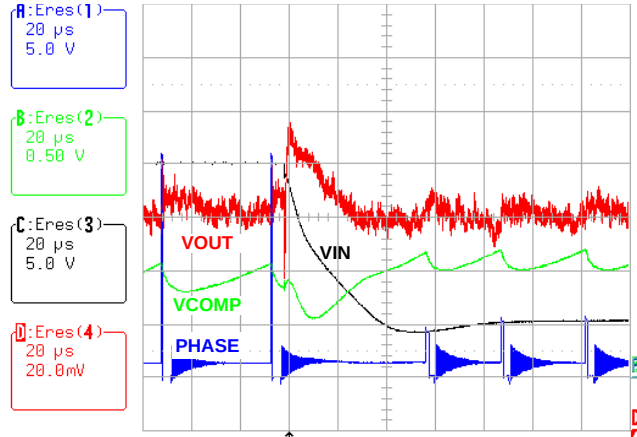
FIGURE 13. LINE TRANSIENT: 20V TO 7V STEP, 100mA LOAD
