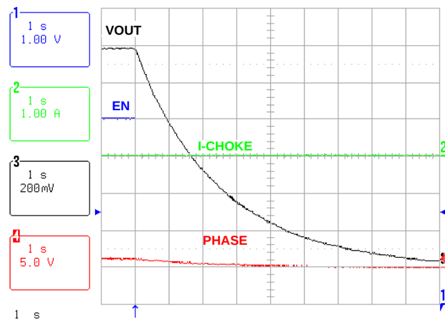
FIGURE 6. SHUTDOWN: EN FALLING, NO LOAD
