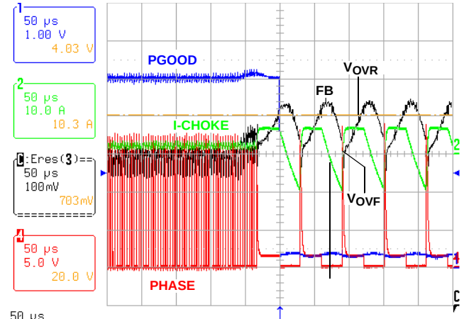
FIGURE 14. OVERVOLTAGE PROTECTION: SHORT ACROSS HIGH-SIDE MOSFET DRAIN-SOURCE, 2A DC STATIC LOAD
