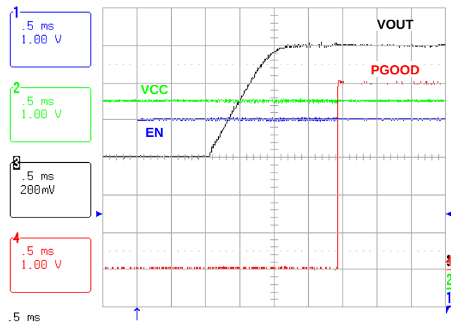
FIGURE 2. SOFT-START: NO LOAD, 50% VOUT-PREBIAS
