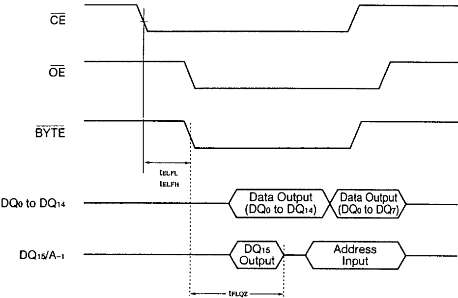
Figure 12 \overline{BYTE} Timing Diagram for Read Operations
