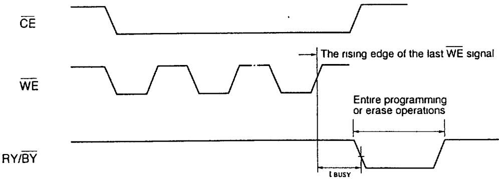
Figure 10 RY/\overline{BY} Timing Diagram during Program/Erase Operations
