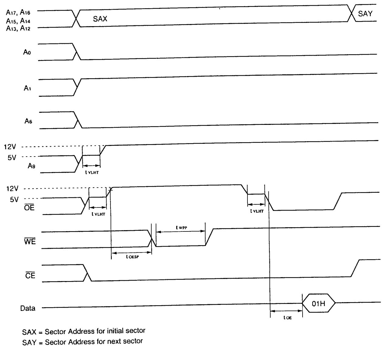
Figure 14 AC Waveforms for Sector Protection
