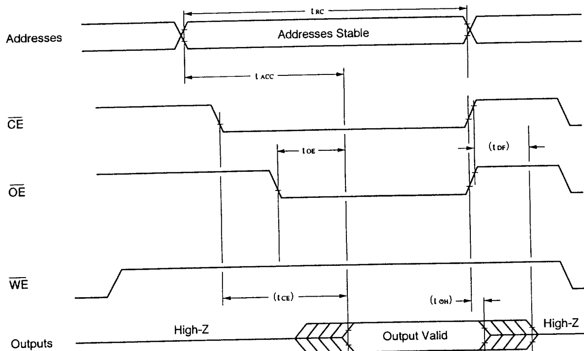
Figure 4 AC Waveforms for Read Operations
