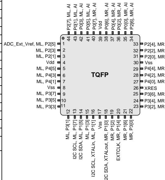
Figure 4. Pin Diagram
