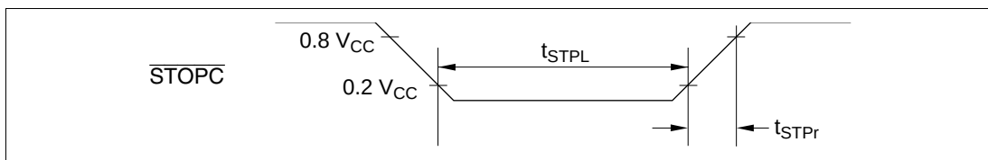
Figure 25-22 \overline{STOPC} Timing (HD404358 and HD404358R Series)
