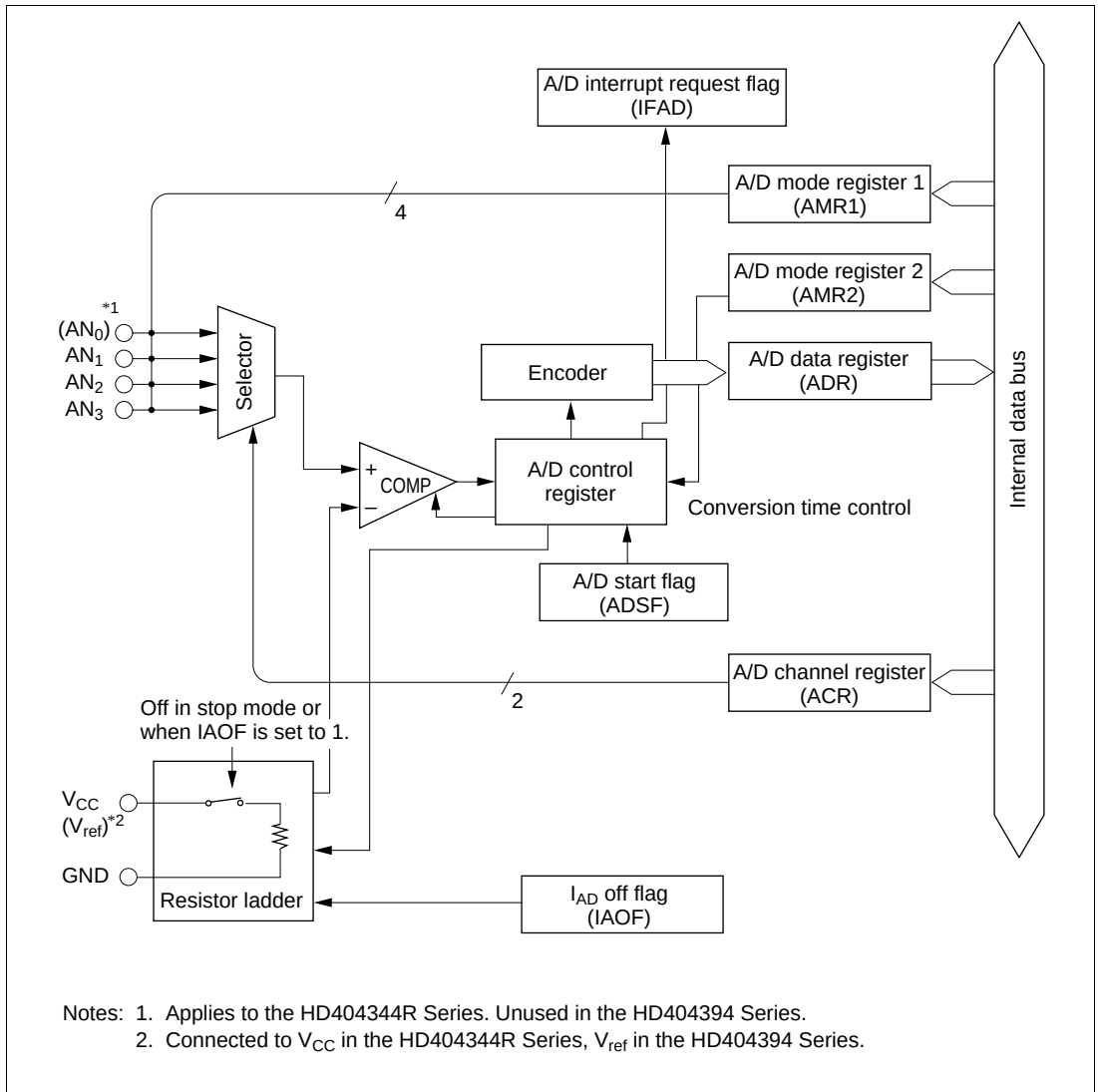
Figure 15-1 (a) A/D Converter Block Diagram (HD404344R/HD404394 Series)
