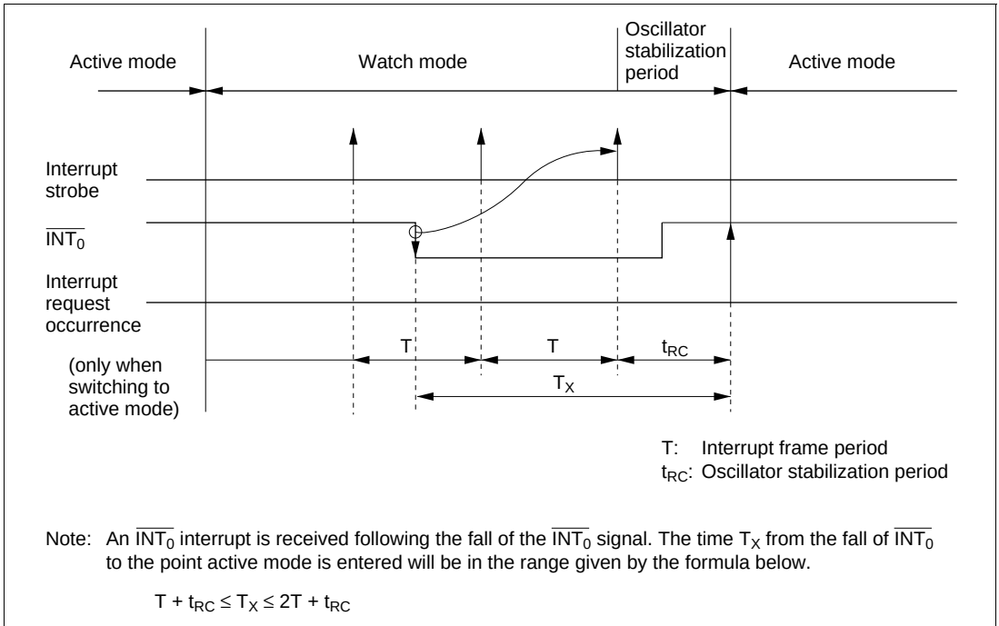
Figure 6-5 Watch Mode to Active Mode Transition Timing
