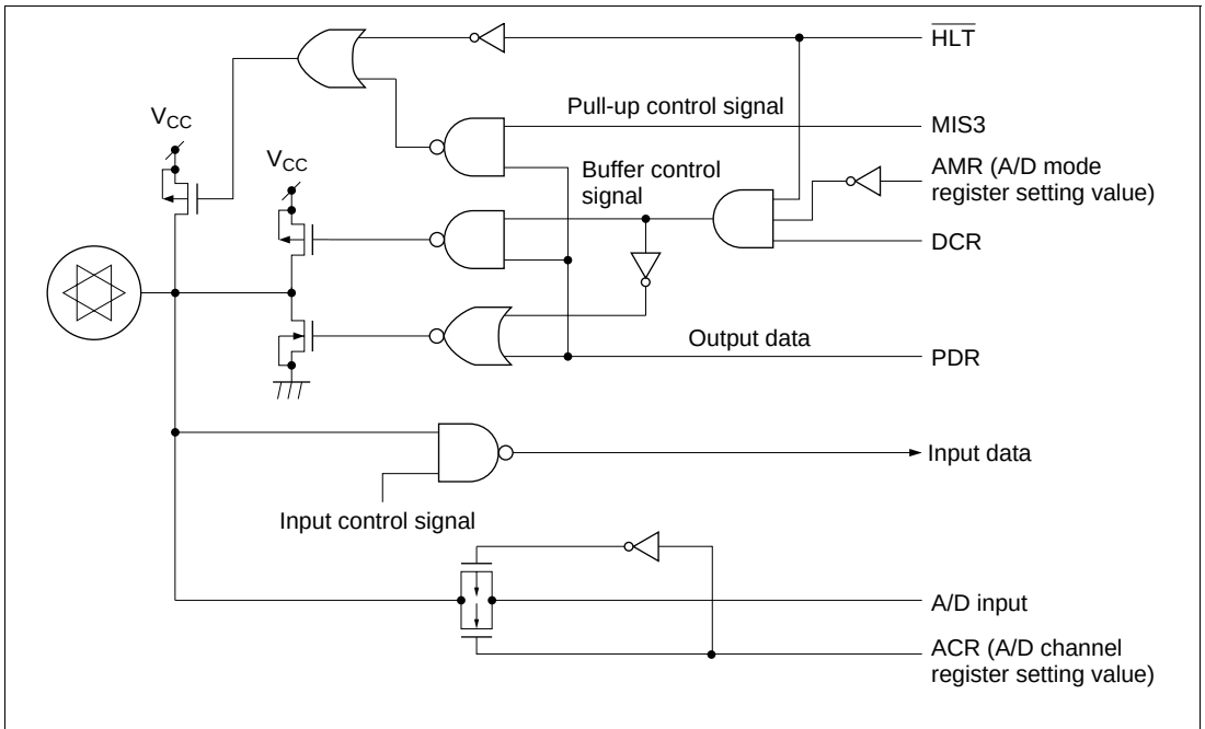
Figure 15-5 R Port/Analog Input Shared Function Pin Circuit
