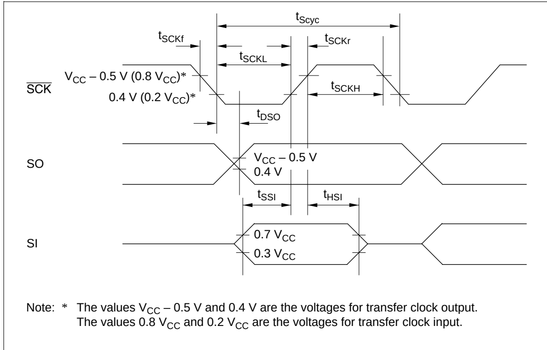
Figure 25-23 Serial Interface Timing (HD404358 and HD404358R Series)
