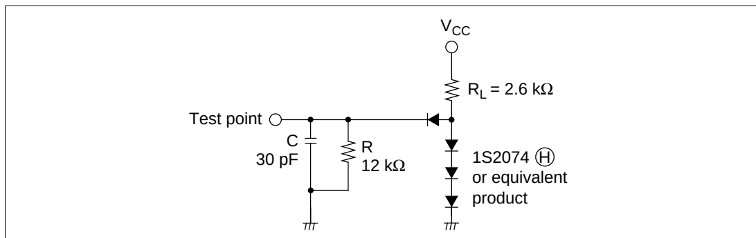
Figure 25-24 Timing Load Circuit
