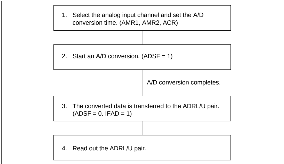
Figure 15-2 A/D Conversion Operation Sequence
