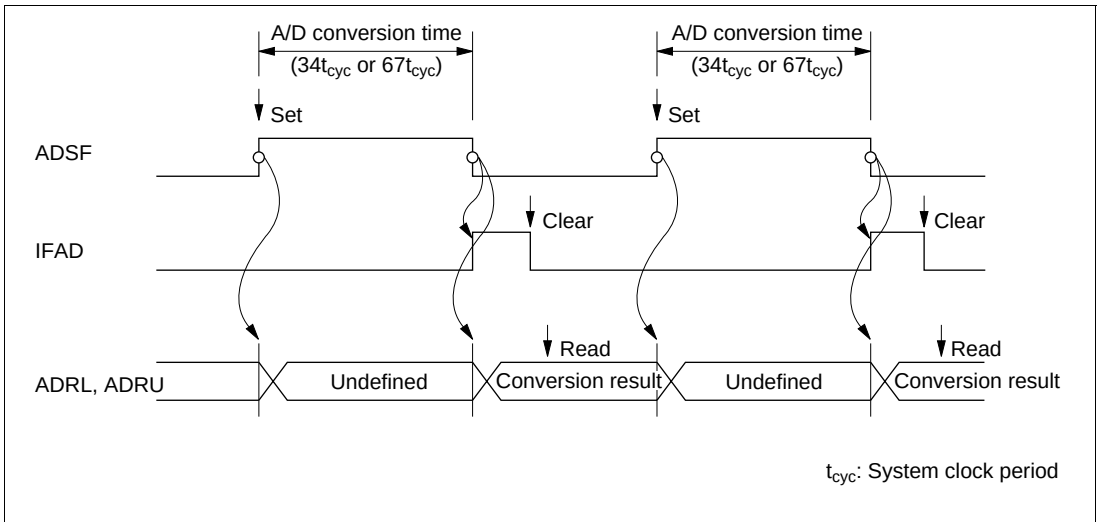
Figure 15-3 A/D Converter Operation Timing Chart
