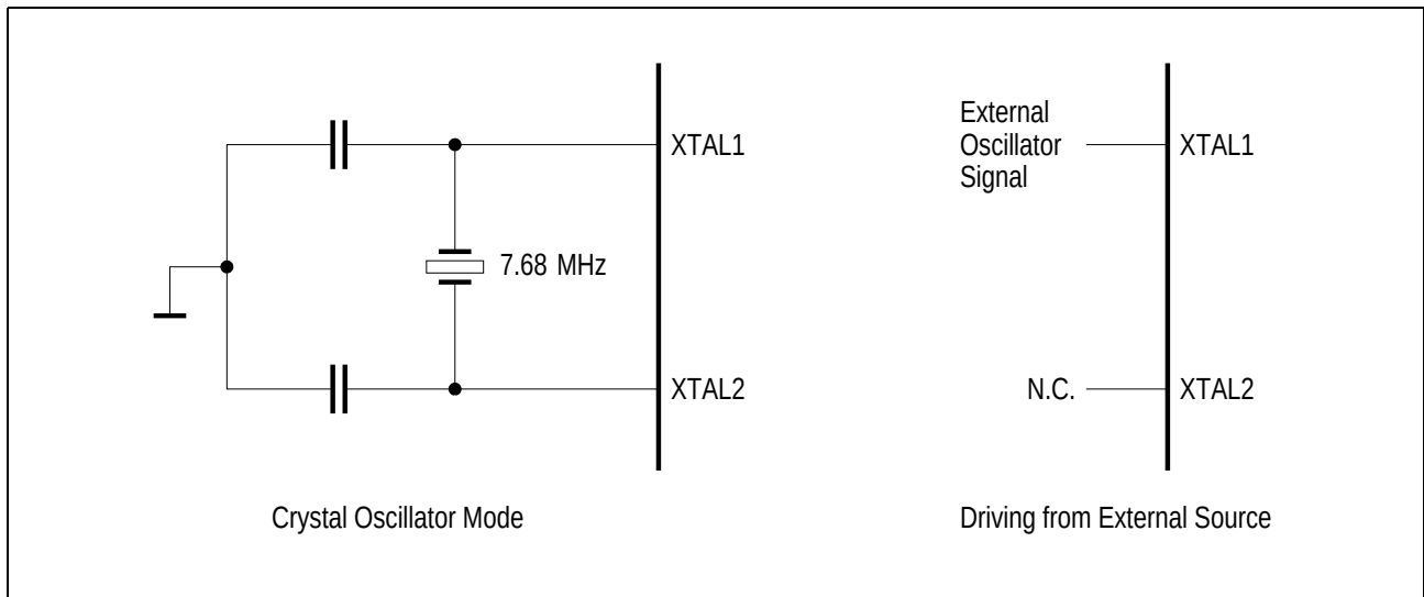
Figure 82 Oscillator Circuits
