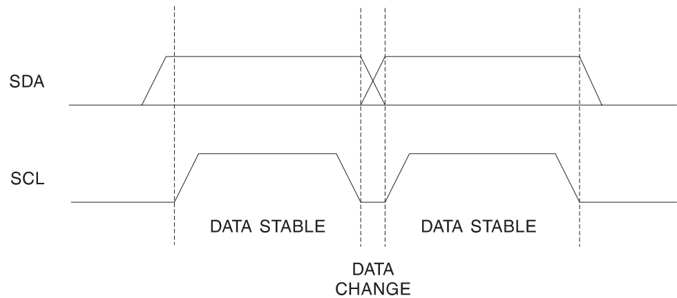
Figure 3. Data Validity
