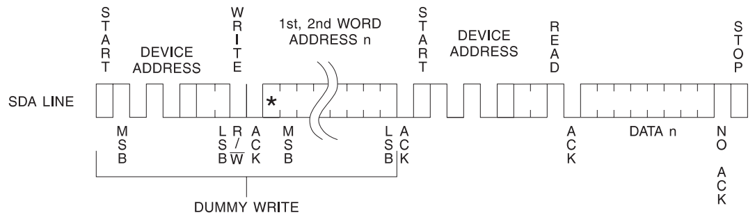
Figure 10. Random Read
