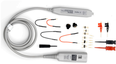
N2819A 800-MHz, 15-V differential probe
