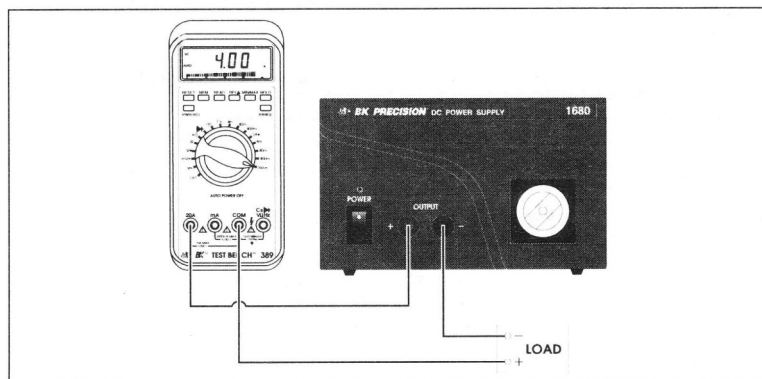
Figure 4 Measuring Output Current
