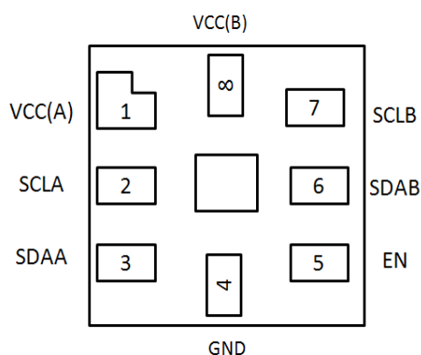
UQFN1.6x1.6-8L(Top view)
