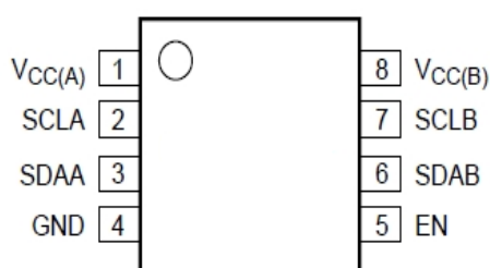
MSOP-8 and SOIC-8
