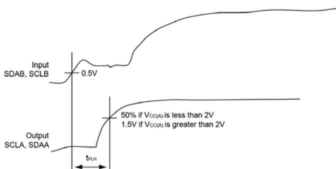
Figure 4: Propagation Delay
