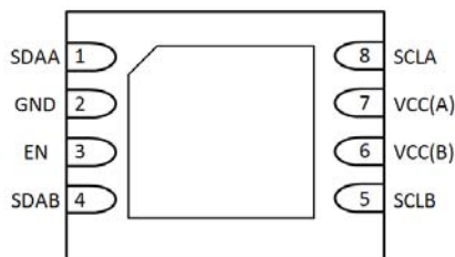
MSOP-8 and SOIC-8
