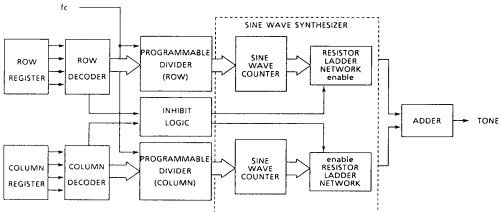
Figure 3-4. Configuration of DTMF Generator
