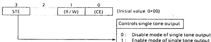
Figure 3-5. TONE command register
