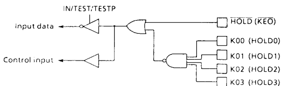
Figure 4-1. Hold control circuit
