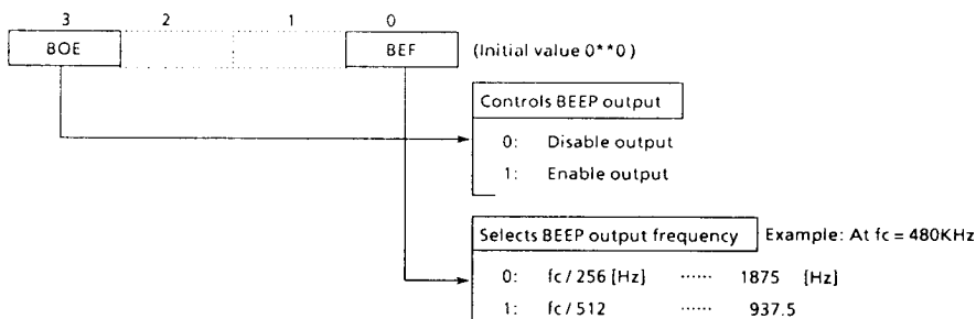
Figure 3-11. BEEP Output Control Command Register
