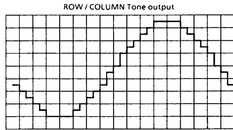
Figure 3-8. Single tone waveform
