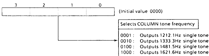
Figure 3-6. ROW, COLUMN Register
