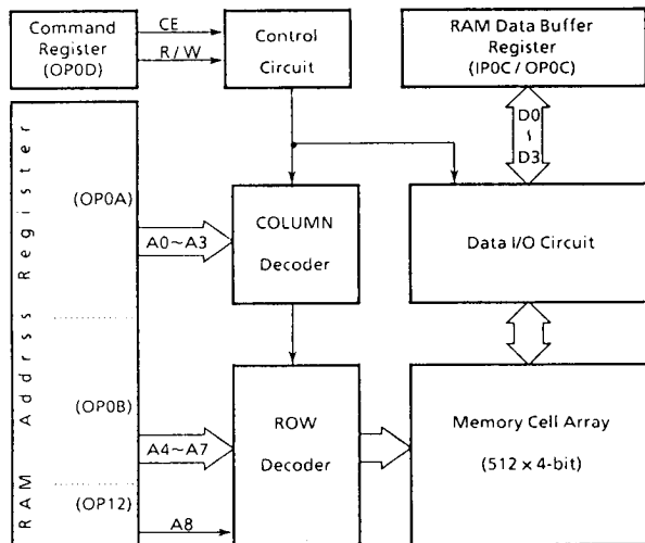
Figure 2-1. Block Diagram
