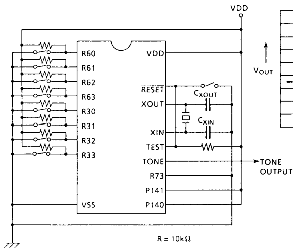
Figure 3-7. Tone test circuit
