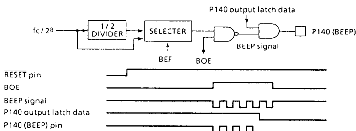
Figure 3-10. BEEP Output Circuit Configuration and Timing Chart
