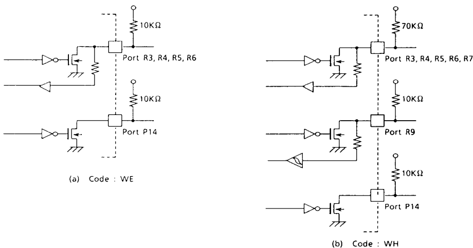
Figure 2. I/O code and external circuitry
