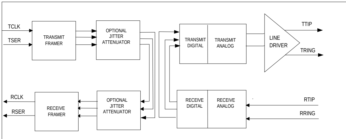
Figure 8-25. Dual Loopback
